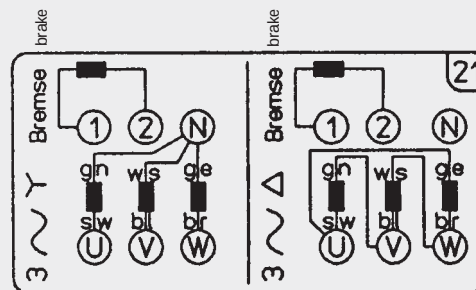
DR 52.0/62.0/ASTO DR 52.1/62.1/ASTO
