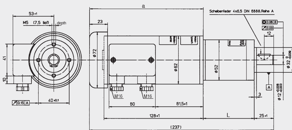
MOTORTYPES DIM. MASS a 62.1x60 146.5 62.1x60 ASTO 176 GEAR UNIT STAGES GETRIEBESTUFEN DIM. I MASS I 1stage 1stufig 50 2stage 2stufig 65.5 3stage 3stufig 80.5
