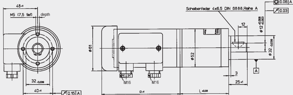
MOTORTYPES DIM. MASS a 52.1x30 106.5 52.1x60 136.5 52.1x30 ASTO 136 52.1x60 ASTO 166 GEAR UNIT STAGES GETRIEBESTUFEN DIM. I MASS I 1stage 1stufig 50 2stage 2stufig 65.5 3stage 3stufig 80.5
